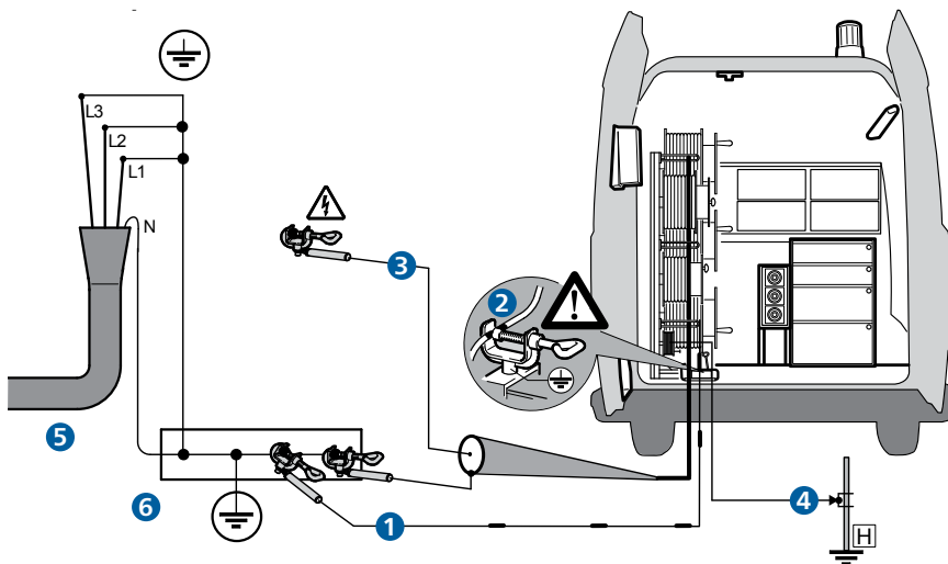
➤ connection of cable fault location system including earth loop control and auxiliary earth monitoring system
