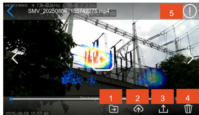
6.2.2-Video Review
