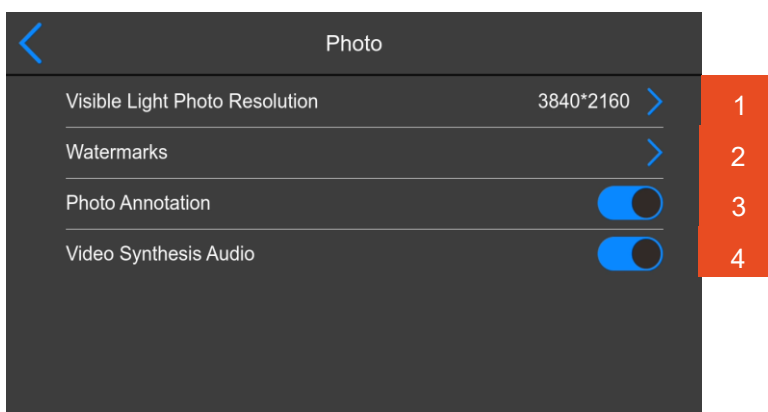
8.5.1-Photo Configurations
