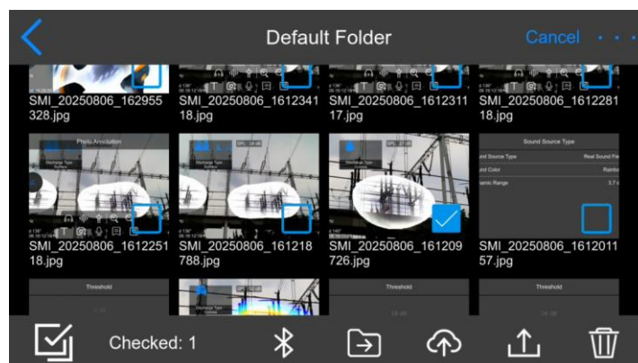
6.1.1.2-Select Folder
