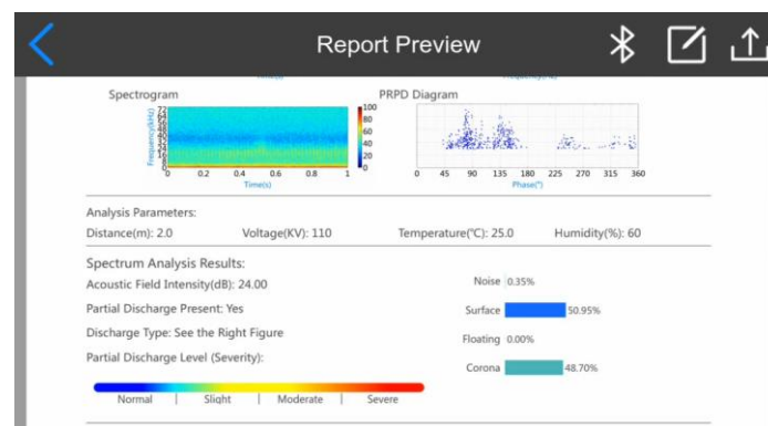
7.2-Report Preview
