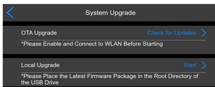
8.8.2-System Upgrade
